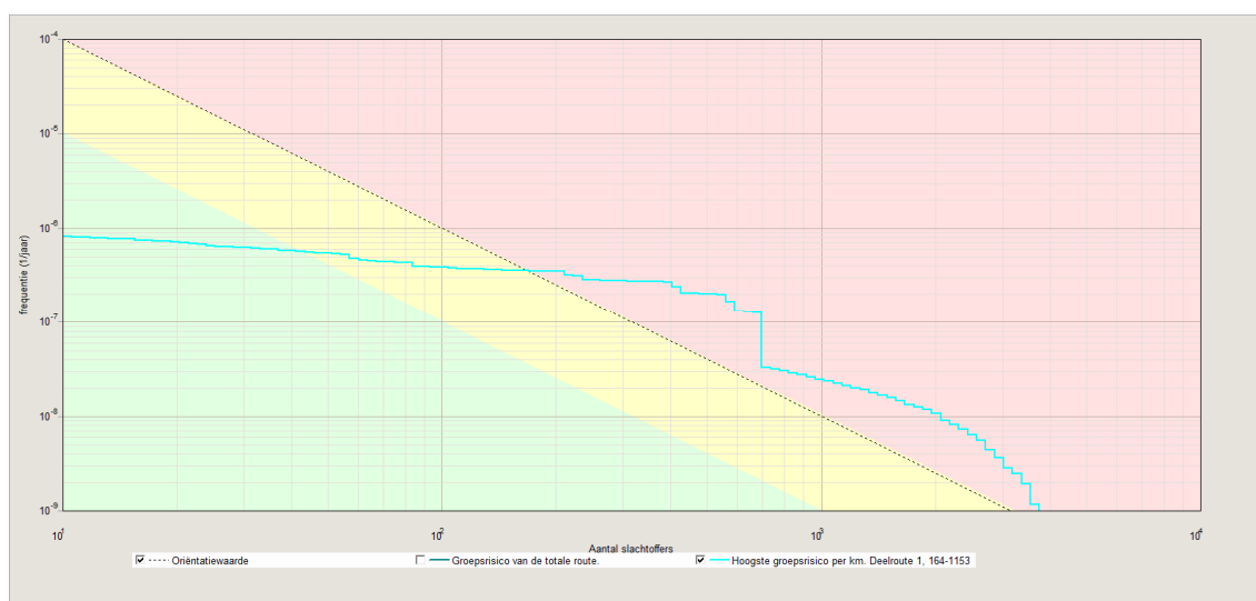
Figuur 39: FN-curve N270 in autonome situatie
